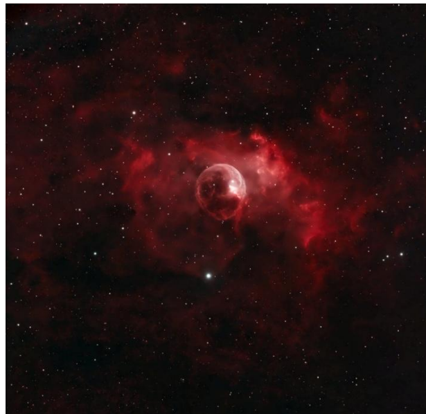
Figure 4: The Bubble Nebula, imaged by the author October 2024:
