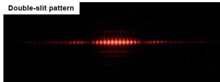
Figure 9: Interference pattern of incident light in a double-slit experiment. By Jordgette - Own work, CC BY-SA 3.0, https://commons.wikimedia.org/w/index.php?curid=9529698 :
