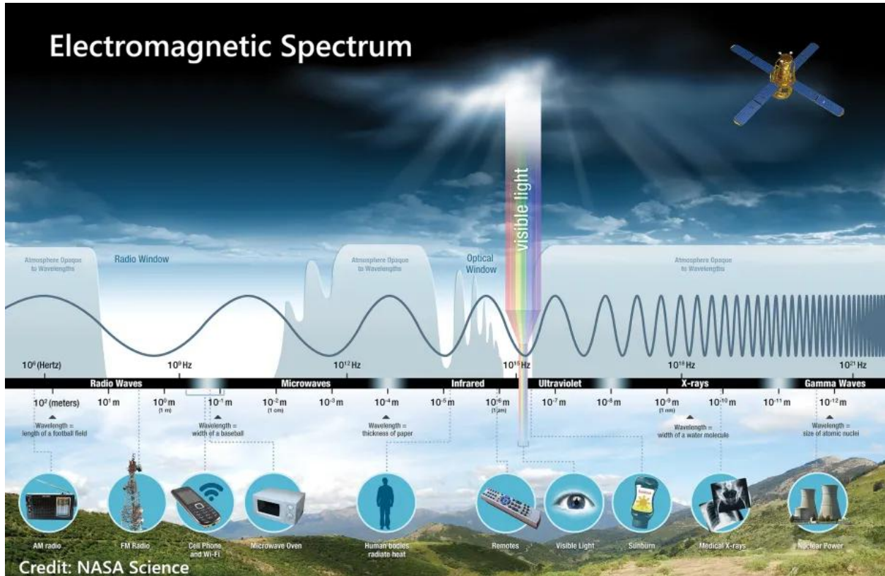
Figure 3: The electromagnetic spectrum, with the narrow band of visible light highlighted in colors:
