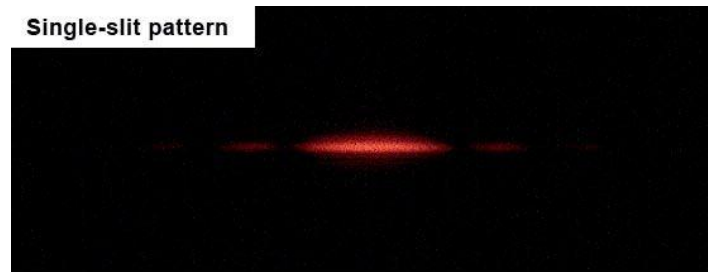
Figure 8: Photograph of incident light in a single-slit experiment. By Jordgette - Own work, CC BY-SA 3.0, https://commons.wikimedia.org/w/index.php?curid=9529698 :
